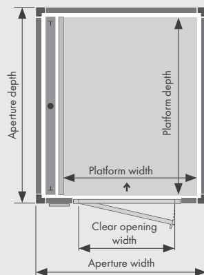
Aluminium structure
